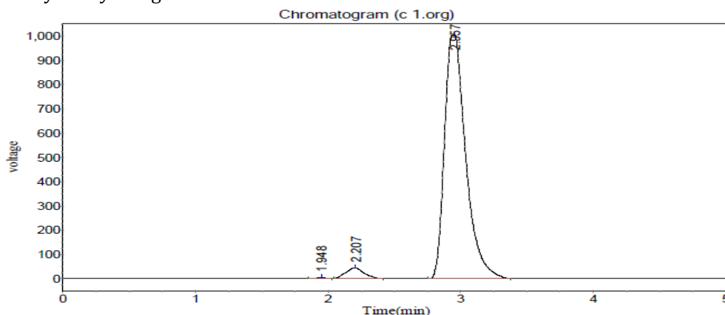
Fig.2 chromatographic trial 1
